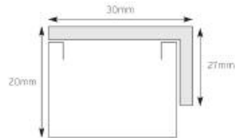
STANDARD HEADRAIL All dimensions are inclusive of brackets.
